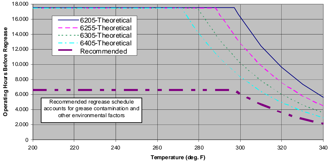
Regrease Schedule - 6005-Series Unions @ 500 RPM Kluber Barrierta L55/2 or Lubcon Turmotemp II/400 or Dupont Krytox XHTRUF grease.
