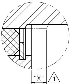
"X" SEAL WEAR DETAIL A (4:1)
