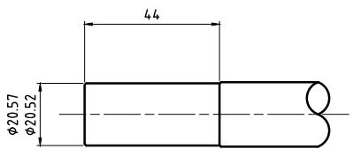
SYPHON PIPE DETAIL
