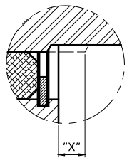
"X" SEAL WEAR DETAIL A (5:1) △
