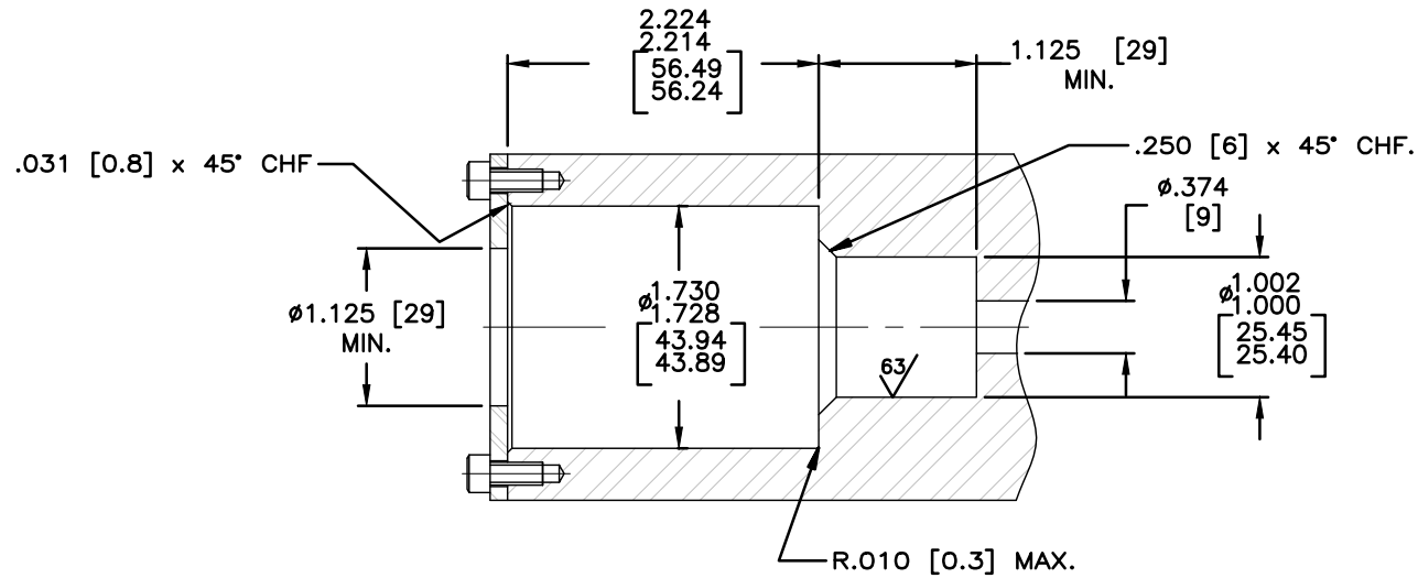
CUSTOMER BORE DETAIL SCALE = 1:4
