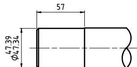
PIPE DETAIL
