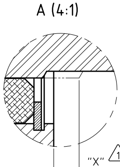
"X" SEAL WEAR DETAIL
