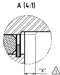
SEAL WEAR DETAIL
