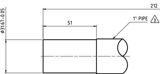
CUSTOMER SIPHON PIPE END DETAIL
