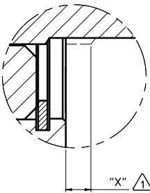
SEAL WEAR DETAIL A (5:1)
