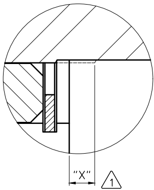
SEAL WEAR DETAIL A (5:1)
