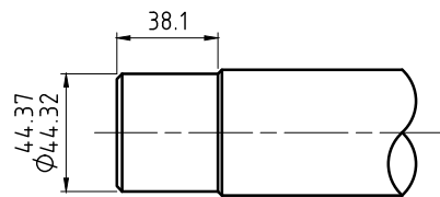
1 PIPE DETAIL
