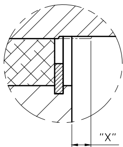
3 SEAL WEAR DETAIL A (5:1)
