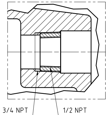
DETAIL B ③
